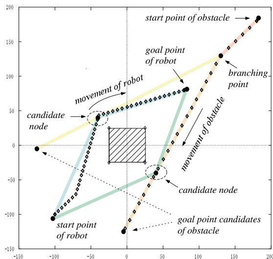
Fig. 11: Simulation result for the case of path ambiguity of a moving obstacle.
