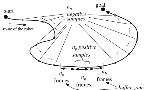
Fig. 3 Making training data for localization SVM
