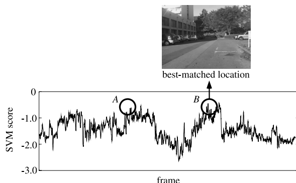
Fig. 7 Localization failure when using a conventional camera
