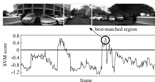
Fig. 6 Result of a localization experiment in our campus
