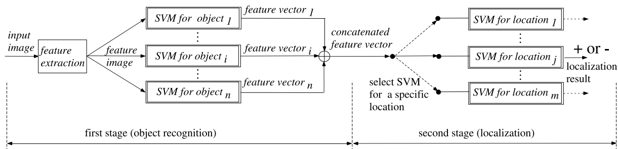
Fig. 1 Two-stage localization using SVMs
